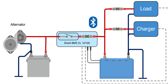
The Smart BMS CL 12/100 will turn loads and chargers off via "load disconnect" and "charge disconnect" signals. It also controls and limits the alternator
